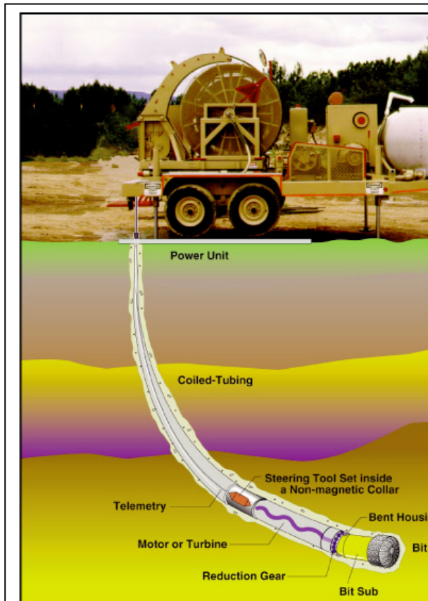
Fig. 3. Early Representation of the Microdrilling Rig and Drilling Assembly Concept
