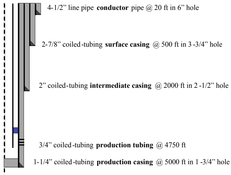
Fig. 14A. Microwell Completion Concept A that includes an intermediate casing string.
