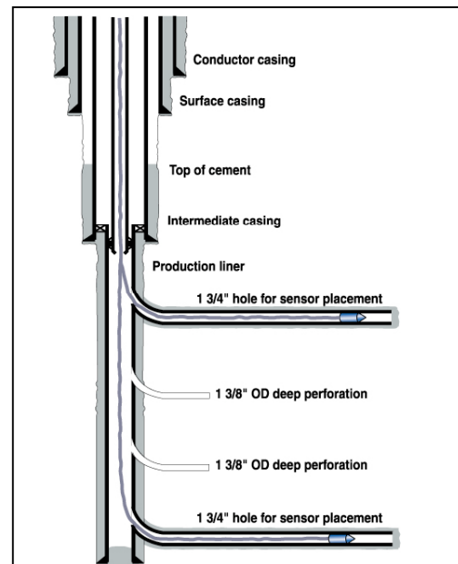
Fig. 2. Through-tubing microlateral and deep perforation concept using microdrilling technology. The DeepLook Consortium pursued microdrilling as means to place sensors away from the well bore to locate bypassed oil and then drill to and produce bypassed oil from “ultra-deep” perforations produced by microdrilled and microlateral completions.
